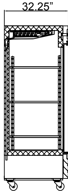
SECTION VIEW
