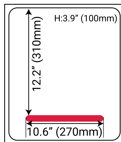
Seal Bar Configuration
